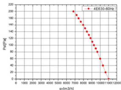
FLOW RATE CURVE (风量曲线):
