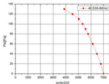
FLOW RATE CURVE (风量曲线):
