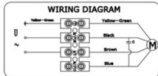
WIRING DIAGRAM (接线图):
