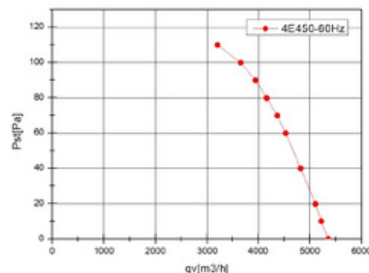
FLOW RATE CURVE (风量曲线):
