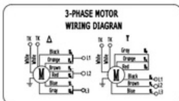
WIRING DIAGRAM (接线图):
