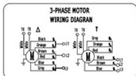
WIRING DIAGRAM (接线图):
