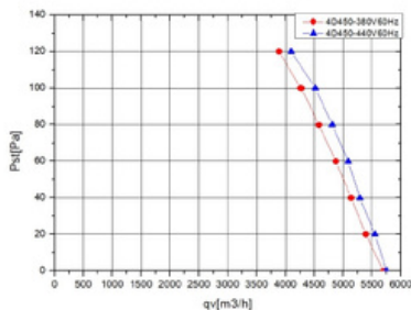
FLOW RATE CURVE (风量曲线):
